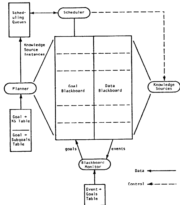
FIGURE 2: Goal-Directed Hearsay-II Architecture
