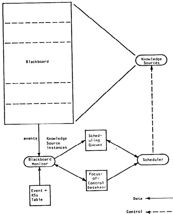
FIGURE 1: Data-Directed Hearsay-II Architecture
