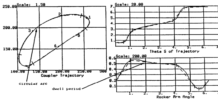
Figure 5: Curvature of The Coupler Curve and Angle of The Rocker Arm
