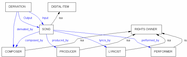
Figure 1: Excerpt of the MPEG-21 related ontology supporting music retrieval and rights management aspects
