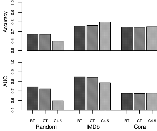
Figure 8. Tree accuracy and AUC.
