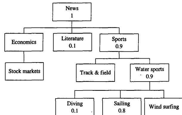
Figure 6. Simplified example of a hierarchical model.
