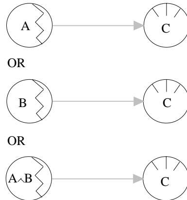
Fig. 12: Alternative representation for rule: IF A OR B THEN C
