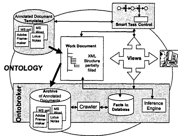
Figure 1: Reactive Agent-Support Framework
