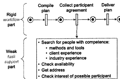
Figure 2: Integrating workflow and context-based views
