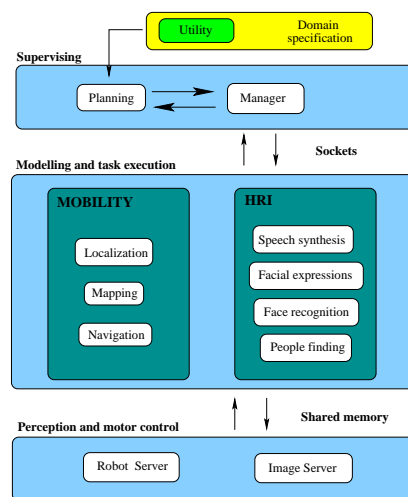
Figure 2: Control Architecture
