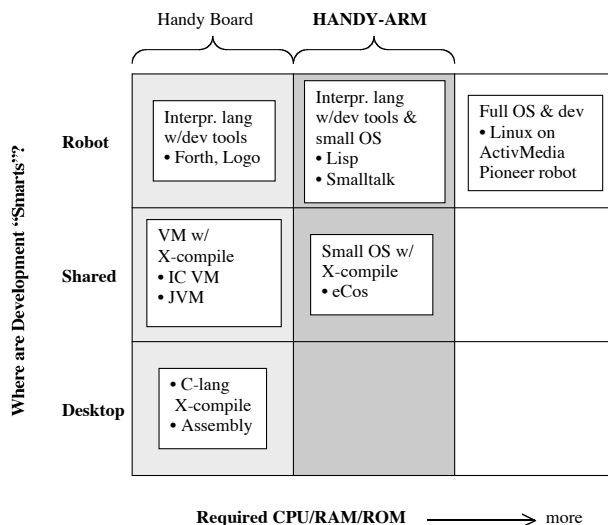
Figure 2: Location of Development Smarts Versus CPU Power
