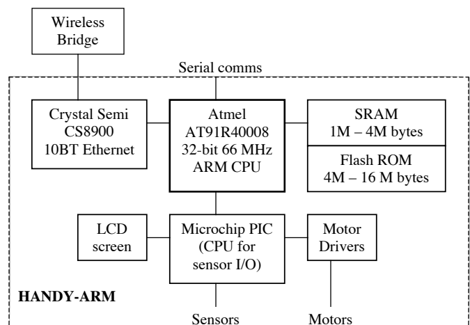
Figure 3: Block Diagram of Handy-Arm Board
