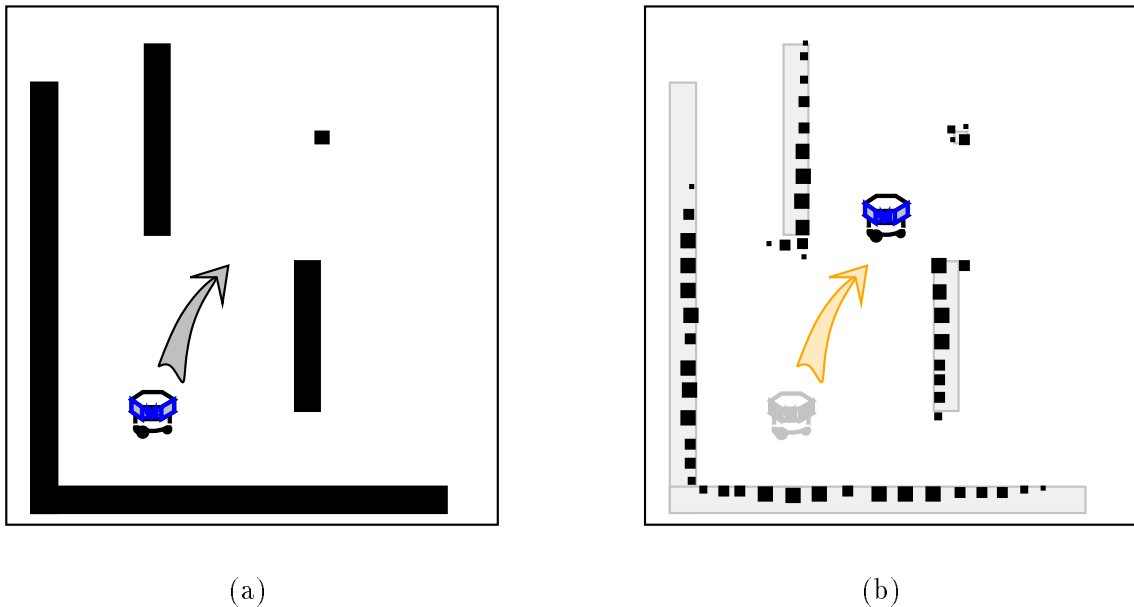
Figure 6: CARMEL constructs a histogram grid as it moves through unfamiliar territory, to collect data from ultrasonic range sensors. In (a) above, CARMEL is at a start location, and heading roughly northeast. In (b), CARMEL has moved, collecting sonar readings in the process, and formed a histogram grid. The histogram grid is illustrated as dark squares; the larger the square, the higher the certainty of an object at that location.
