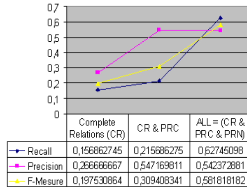
Figure 14: Recall, Precision and F-Measure for a threshold at 0.3
