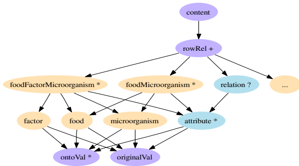
Figure 11: Extract of SML DTD (risk assessment)
