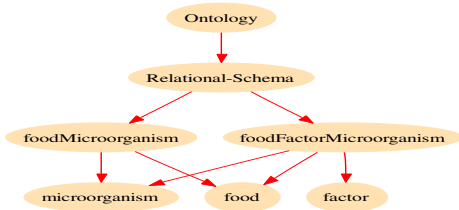
Figure 10: Extract of a risk assessment ontology
