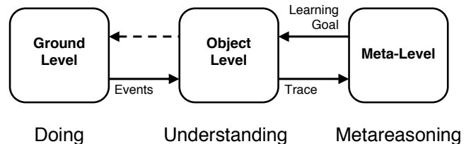
Figure 4. Introspective monitoring in Meta-AQUA
