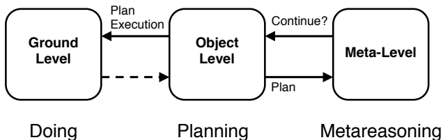
Figure 3. Classical metareasoning (from Russell and Wefald 1991)
