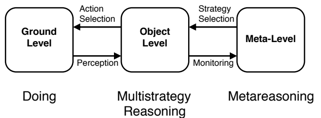
Figure 6. Example integrated model of self
