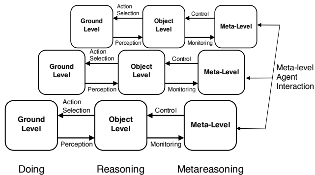
Figure 5. Meta-level reasoning among multiple agents
