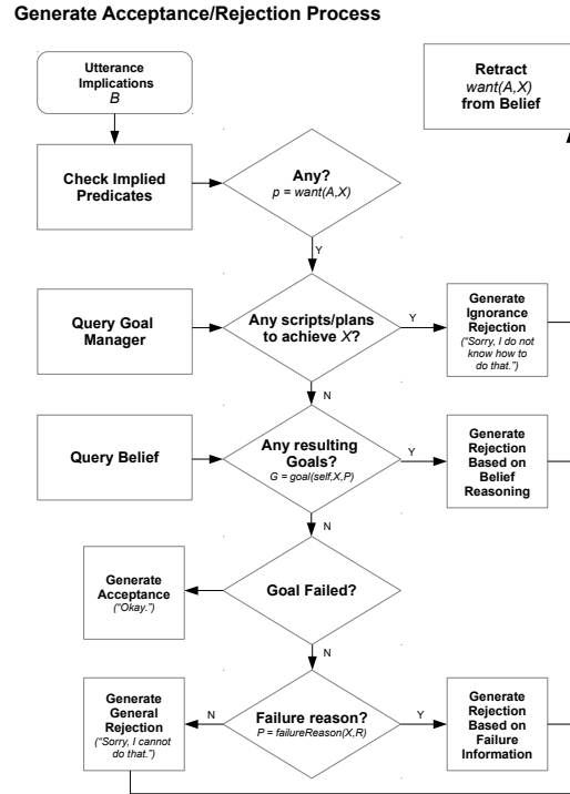
Figure 1: Directive acceptance/rejection reasoning process in the current DIARC/ADE NL architecture.
