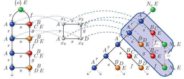
Figure 3: An example for the correspondence between entailment and quasi-entailment.
