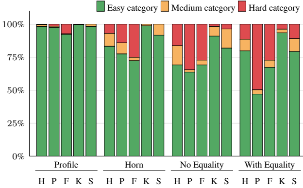
Figure 4: Percentage of Easy, Medium and Hard Ontologies per Ontology Group for HermiT (H), Pellet (P), FaCT++ (F), Konclude (K), and Sequoia (S)
