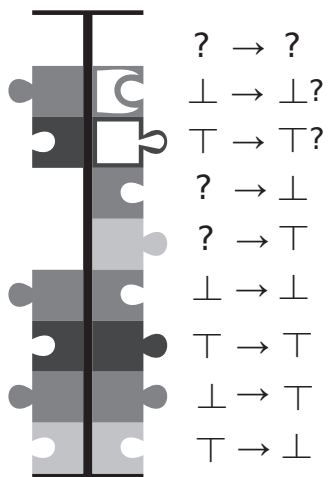
Figure 2: Possible cases of precondition and effects using DOVETAIL notation.
