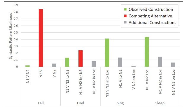
Figure 3: The model’s likelihoods for the top three values for the syntactic pattern for each of four verbs: two has-CA, find and fall on left; and 2 no-CA, sing and sleep on right.
