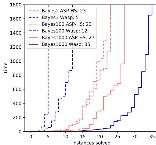
Figure 4: Comparison of ASP-HS with Wasp on the Bayes benchmark family.
