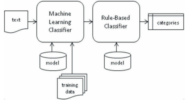
Figure 1. Logical architecture
