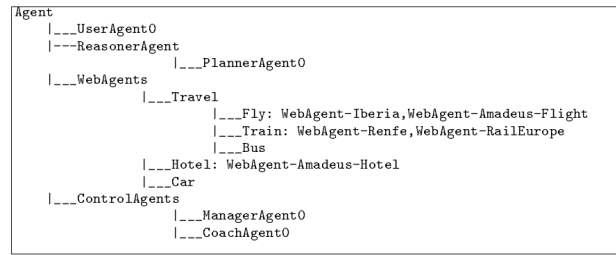
Figure 5: Agents Hierarchy. It describes all the available agents in MAPWEB and their information gathering skills.
