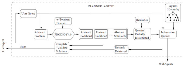
Figure 2: Planning Process developed by the PlannerAgent. The user query is transformed into an abstract planning problem, which is subsequently solved by PRODIGY4.0. Each solution is partially instantiated by means of domain dependent heuristics. Every operator in a solution generates several WEB queries, which is sent to the appropriate WebAgents by using the agent hierarchy. The agents return several records, that are used to complete and validate the abstract solutions.
