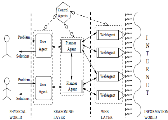
Figure 1: MAPWEB three-layer architecture.
