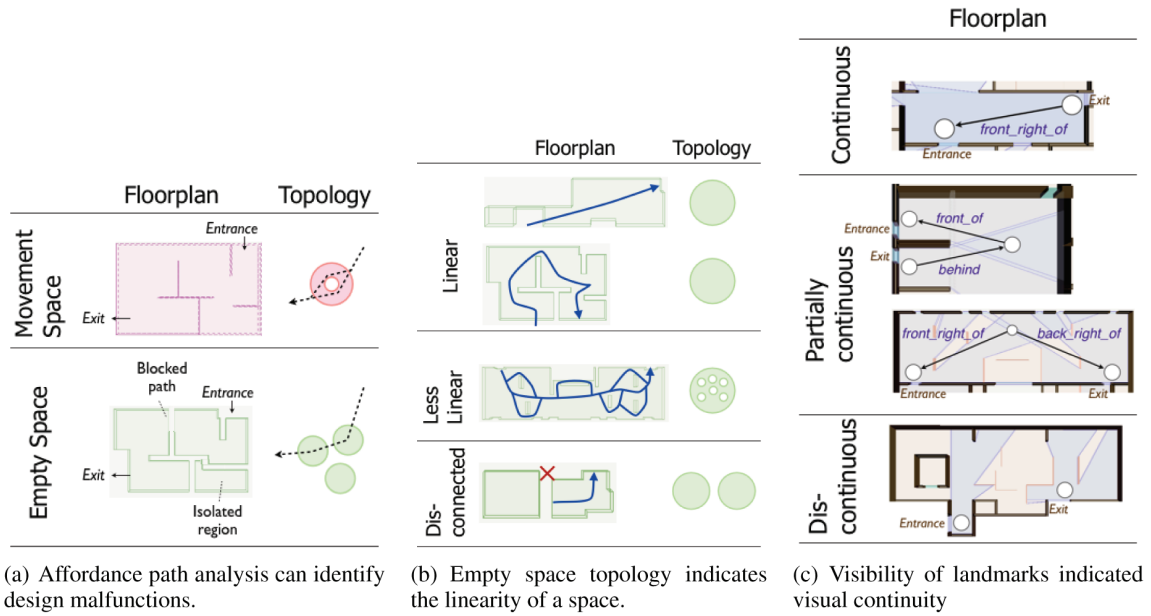
Figure 6: Affordance Paths, and Navigation Linearity and Visual Continuity
