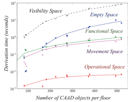
Figure 11: Time taken for Design Typology Computation
