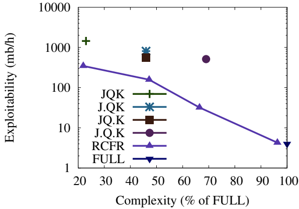
Figure 2: Exploitability of final strategies after 100000 iterations of RCFR, unabstracted CFR (FULL), or chance sampling CFR (JQK, J.QK, JQ.K, and J.Q.K). The horizontal axis shows the complexity of the solution method as a percentage of the size of the unabstracted game. RCFR’s complexity is the size of the regression tree while the complexity of a conventional abstraction is the size of its abstract game.
