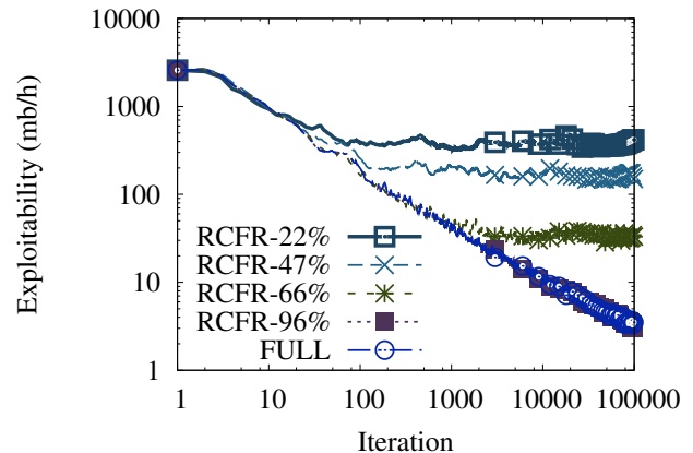
Figure 1: Convergence of RCFR using various error thresholds (complexity limitations) compared with CFR on the unabstracted game (FULL).
