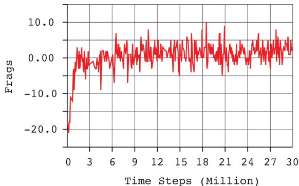
Figure 3: Number of frags achieved during training, run on 2 minute rounds
