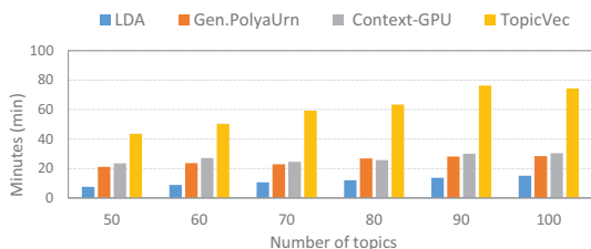
Figure 3: Execution time vs. number of topics.
