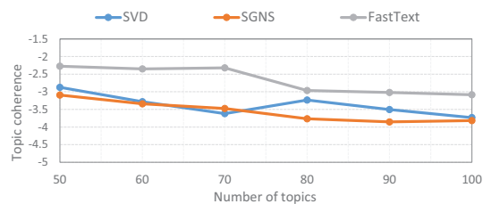
Figure 2: Context-GPU with different word/phrase embedding learning methods vs. number of topics.
