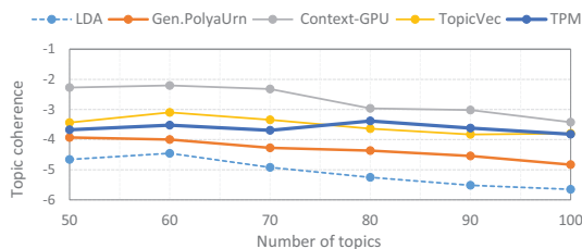
Figure 1: Topic coherences vs. number of topics.
