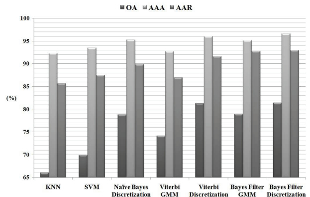
Figure 7: OA, AAA, and AAR of Binary States Classification
