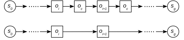
Figure 4: A raw workflow (top) and a final workflow (bottom).
