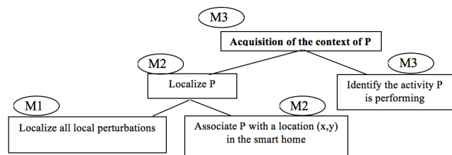
Figure 5 The activation schema associated to the goal "Acquisition of the context of P".
