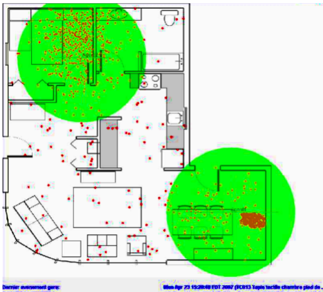
Figure 1 Two localization agents: particles and possible localization area of their user.
