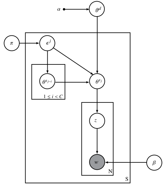
Figure 2: The graphical model of the RATM. \vartheta^{d^i} is the topic distribution of a document. \theta^{s_{j-1}} denotes the topic distribution of a preceding sentence where 1 \leq i < C and C is the length of time windows used in the RABP.
