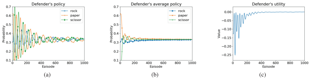
Figure 8: Results of StackGradFP on Rock-Paper-Scissors: (a) Defender's policy at each episode, (b) Defender's average policy at each episode, and (c) Defender's utility at each episode.
