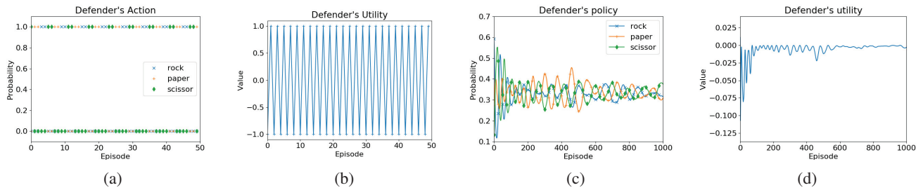
Figure 7: Results of CA and StackGrad on Rock-Paper-Scissors: (a) Defender's actions with CA on RPS, (b) Defender's utility with CA on RPS, (c) Defender's policy with StackGrad on RPS, (d) Defender's utility with StackGrad on RPS.
