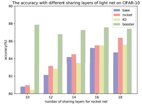
Figure 4: The accuracy with different sharing layers of light net on CIFAR-10
