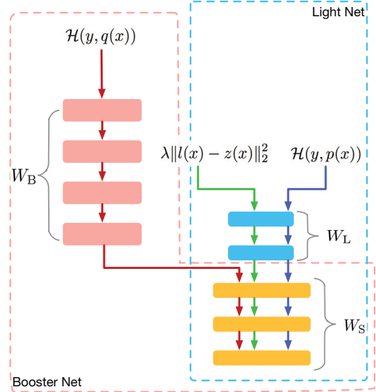
Figure 2: Gradient backward with the gradient block scheme.
