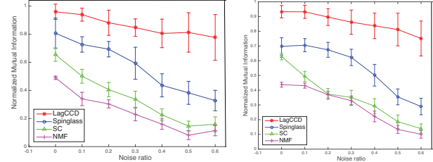
Figure 3: Sensitivity to noise on Dolphin (left) and Political Book (right) data sets
