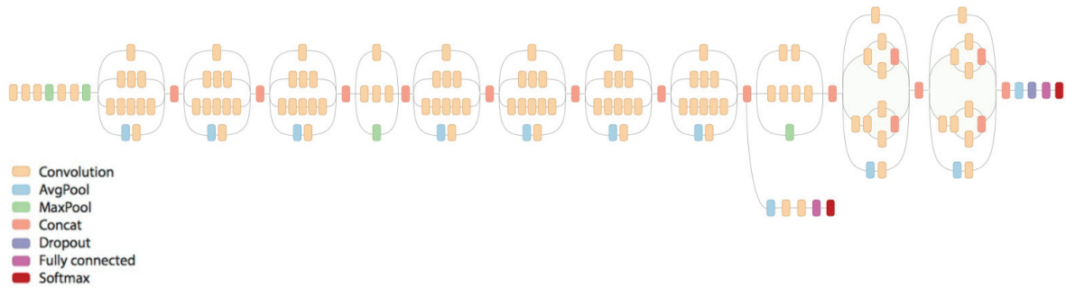
Figure 6: Schematic diagram of Inception-v3 (Shlens 2016).
