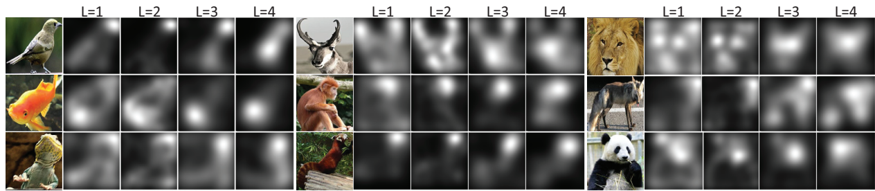
Figure 6: Heat maps of patterns. We use a heat map to visualize the spatial distribution of the top-50% patterns in the L -th layer of the explanatory graph with the highest inference scores.
