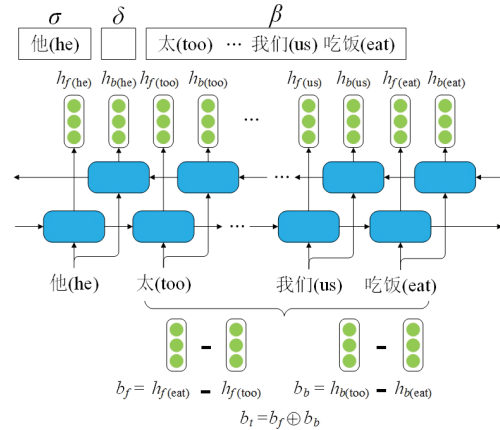
Figure 3: Illustration of Bi-LSTM Subtraction for buffer representation learning. h_f^* and h_b^* indicate the hidden vectors of forward and backward LSTM respectively. b_t is the resulting buffer representation.
