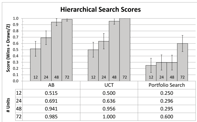
Figure 4: Results of Hierarchical Adversarial Search against Alpha-Beta, UCT and Portfolio Search for combat scenarios with n vs. n units ( n = 12, 24, 48 and 72 ). 60 scenarios were played allowing 40 ms for each move. 95% confidence intervals are shown for each experiment.
