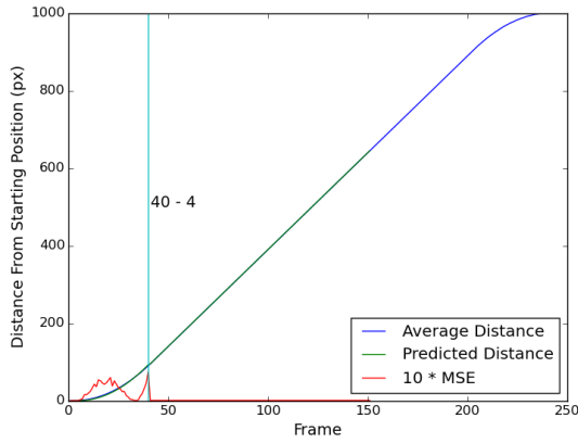
Figure 3: A graph depicting actual and predicted positions as well as prediction errors and the best frame to use for the top speed of the Protoss arbiter.
