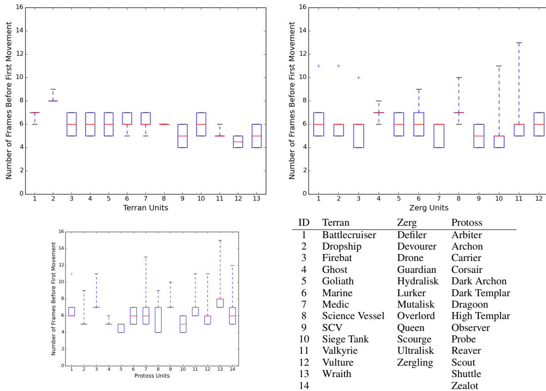
Figure 2: Box plots for the delay between ordering a unit to move and the first change in its position measured in number of game frames. These graphs contain data for all Terran, Zerg, and Protoss units.
