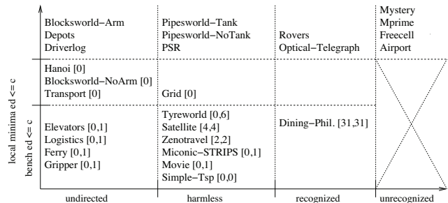
Figure 1: Overview of h^+ topology (Hoffmann 2005).
