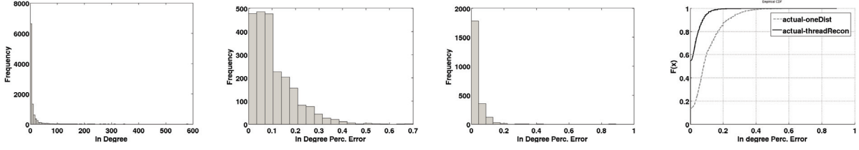
(a) Histogram of the in-degree of all vertices of the actualGraph. (b) In-degree percentage error between the vertices of actualGraph and oneDistGraph, for all vertices with degree \geq 10 . (c) In-degree percentage error between the vertices of actualGraph and threadReconGraph, for all vertices with degree \geq 10 . (d) CDF plot of the in-degree percentage error, comparing the results for oneDistGraph and threadReconGraph.
