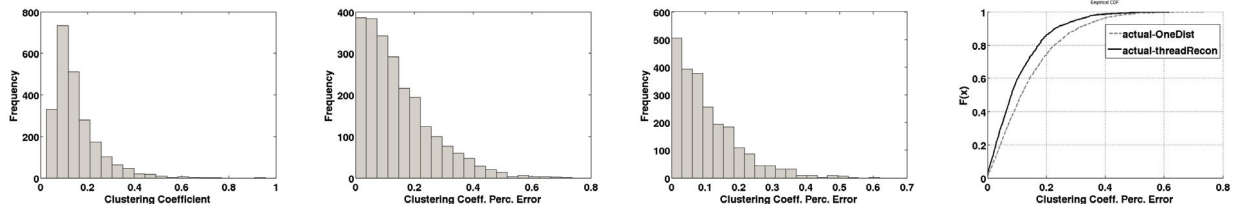
(a) Histogram of the clustering coefficient for the actualGraph. (b) Clustering coefficient per-vertex error between actualGraph and oneDistGraph. (c) Clustering coefficient per-vertex error between actualGraph and threadReconGraph. (d) CDF plot of the clustering coefficient per-vertex error, comparing the results for oneDistGraph and threadReconGraph.
