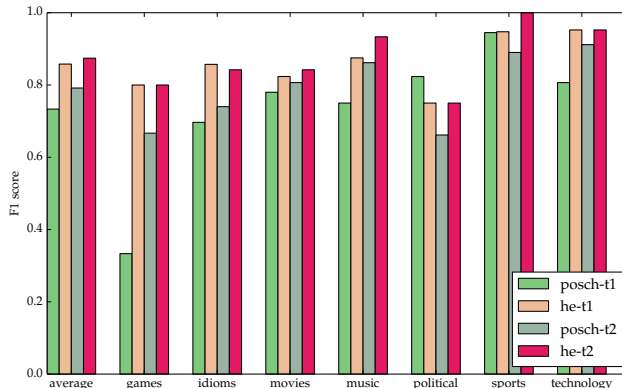
Figure 3: 6-fold cross validation on Posch dataset
