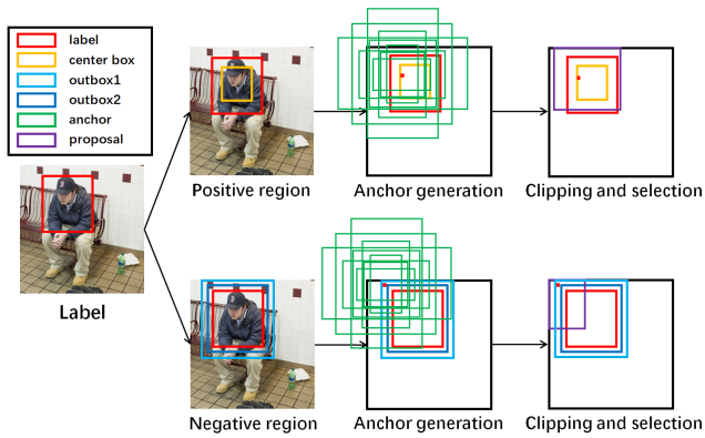
Figure 3: Overview of the predicted anchoring. The center point of positive anchor is included by the center box and negative anchor is included by the outbox1 but excluded by the outbox2. We generate 9 size anchors on all the center point and choose 1 proposal which has the largest/smallest IoU with Graded-Labels as positive/negative sample.
