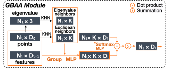
Figure 4: Encoder Module: Geometry Based Attentive Aggregation. The input are point-wise coordinates, colors and features. In GBAA, we aggregate features in both eigenvalue space and Euclidean space, then use attentive pooling to generate the output feature of each point.
