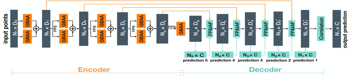
Figure 3: The detailed architecture of our IAF-Net. (N, D) represents the number of points and feature dimension respectively. FPS: Farthest Point Sampling.
