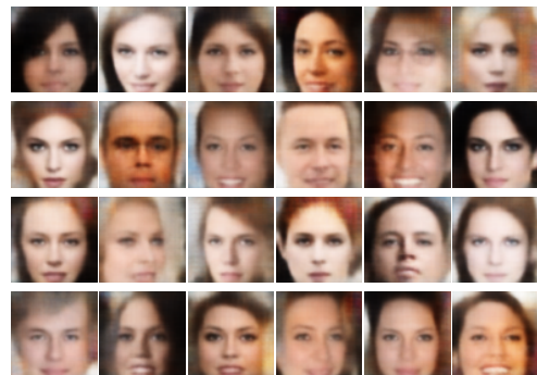
Figure 5: Unconditional Generation of HiABP [E+L] (L = 4) on CelebA
