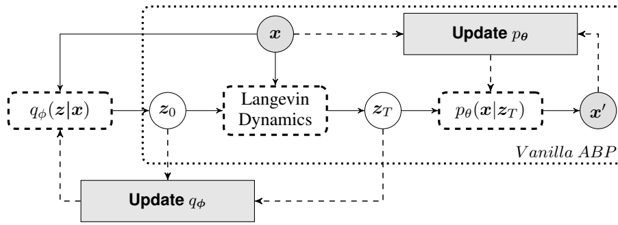
Figure 2: IABP Framework. Different from vanilla ABP ( z_0 \sim \mathcal{N}(0, 1) ), IABP iterates the following three steps: (1) parameterized q_\phi quickly generates initial latent variable z_0 ; (2) Improving latent variable via T -step Langevin dynamics starting from z_0 to obtain z_T ; (3) Updating q_\phi and p_\theta (dashed arrow part). q_\phi is typically updated using Maximum Likelihood estimation (MLE) in unsupervised learning. The MLE provides only a point estimate of the fitted model parameters, while step (2) recovers the entire posterior distribution of the model parameters given in the data by Langevin dynamics. Since the initialization is improved after each q_\phi update, the quality of the Langevin dynamics’ samples also improves.
