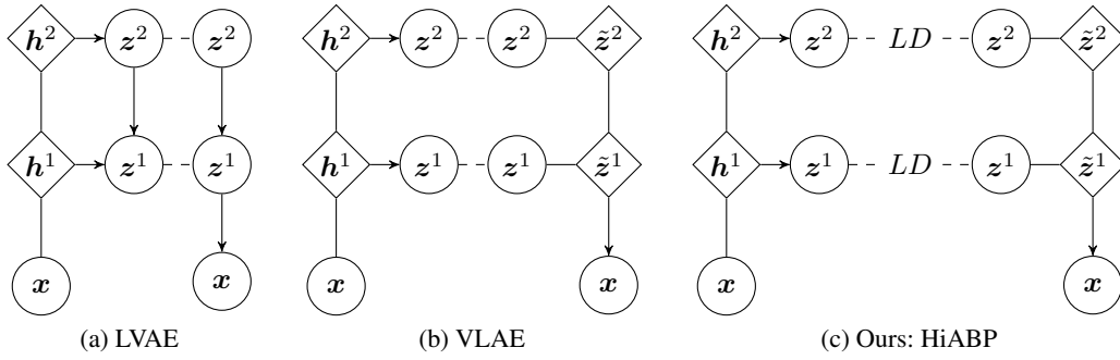
Figure 3: Inference and generative models for LVAE (Sønderby et al. 2016) (left), VLAE (Zhao, Song, and Ermon 2017) (middle) and HiABP (right). Circles indicate stochastic nodes, and squares are deterministically computed nodes. Solid lines with arrows denote conditional probabilities; solid lines without arrows denote deterministic mappings; dash lines indicate regularization to match the prior p(z) . LD represents Langevin dynamics.
