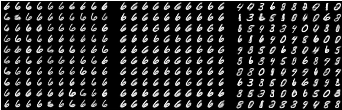
Figure 7: HiABP on MNIST. Each sub-figure corresponds to images generated when fixing latent code on all layers except for one. From left to right, the randomly sampled layer goes from the bottom layer to the top layer. Right panel: the third layer encodes digit identity; Center panel: the second layer encodes digit width; Left panel: the first (bottom) layer encodes stroke width.
