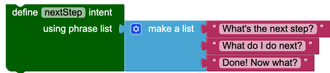
Figure 2: The define intent using phrase list block. Each pink block represents a possible utterance for the intent.
