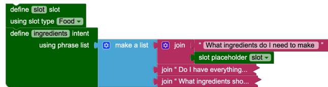
Figure 3: Slot blocks in a VUI definition. Users can define slots of specific types, and use them when defining intents.
