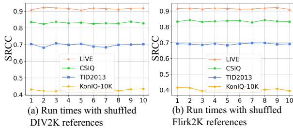
Figure 5: Stability evaluation of our NAR-student. (a)(b) show SRCC results of 10 times tests using randomly shuffled NAR images from DIV2K and Flickr2K, respectively.
