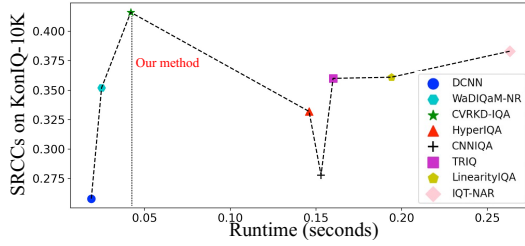
Figure 3: Runtime vs. performance of NR/NAR-IQAs on the real-distorted KonIQ-10K dataset with the Tesla-V100 GPU.
