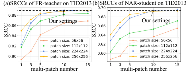
Figure 4: SRCC results with different multi-patch numbers and sizes on TID2013. It's clear that larger patch number and size can capture more local-global information.
