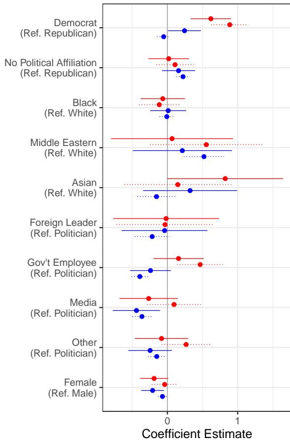
Figure 7: Regression results for the personal insult model for each of the four support measures. Error bars are plus/minus two standard errors. Coefficient estimates are given on the x-axis, model covariates on the y-axis. Coefficients for each of the four different models are given for each variable. Republican (Democrat) measures are colored red (blue), platform (survey) measures are solid (dotted) lines
