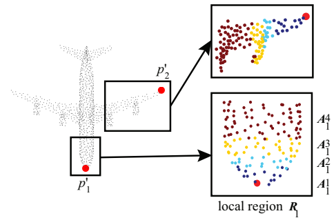
Figure 1: The left is an airplane point cloud with two sampled centroids p'_1 and p'_2 in the red color. The right is the corresponding local regions of p'_1 (below) and p'_2 (above), where different colors represent different area scales within the local region. For example, there are four different scale areas \{A_1^1, A_1^2, A_1^3, A_1^4\} in the local region R_1 centered by p'_1 .
