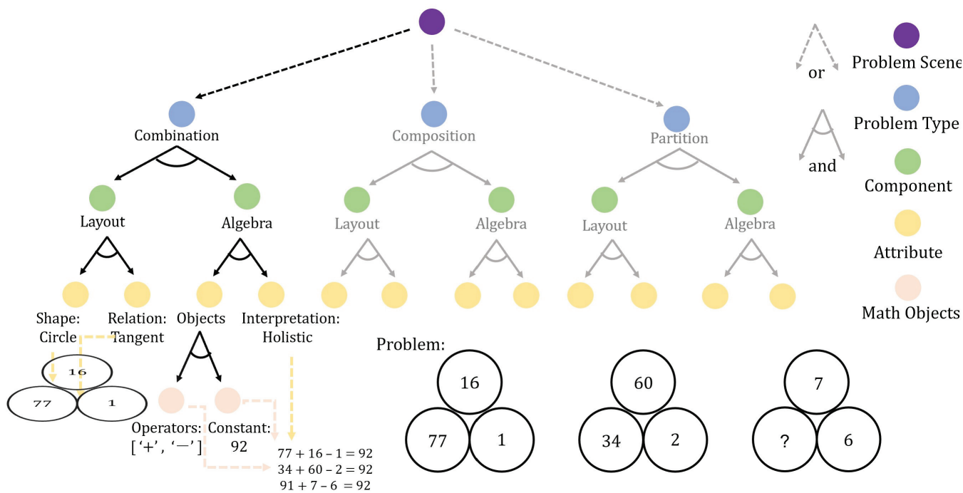
Figure 2: The Machine Number Sense (MNS) dataset creation process. Given grammar production rules together with its attributes, we can generate a test by parsing and sampling an And-Or Graph (AOG).
