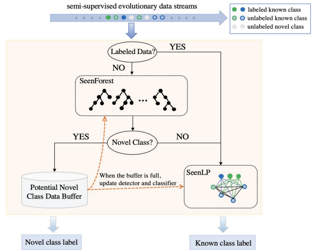
Figure 1: Illustration for our proposed SEEN framework.
