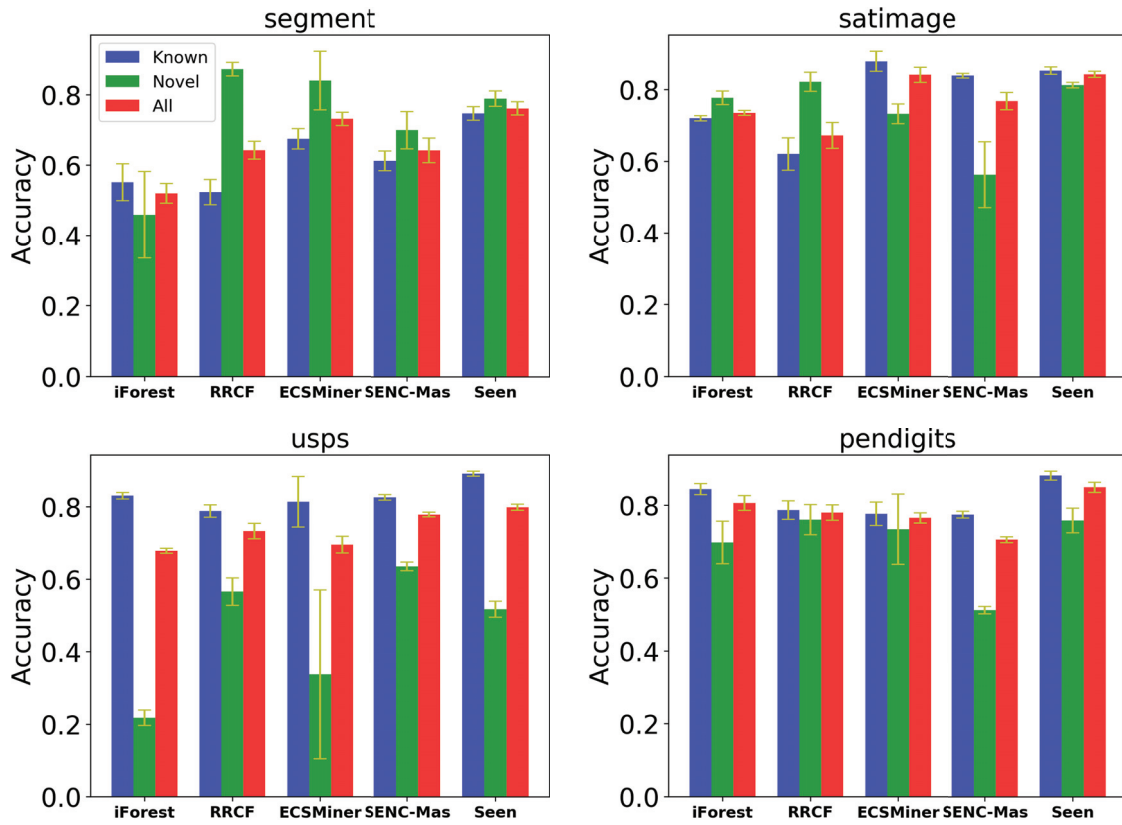
Figure 3: Results of known, novel and all classes, respectively. The yellow segment represents the corresponding variance.
