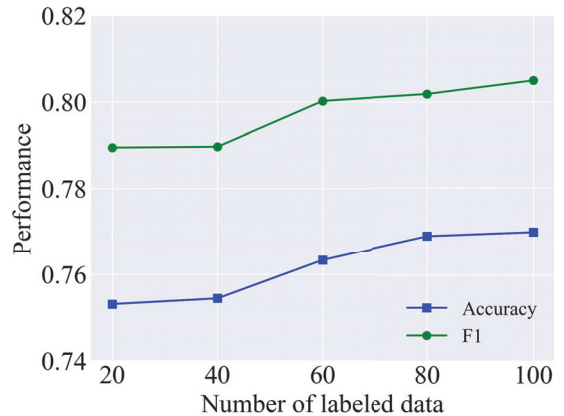
Figure 4: The influence of the number of labeled data in each class on segment dataset.
