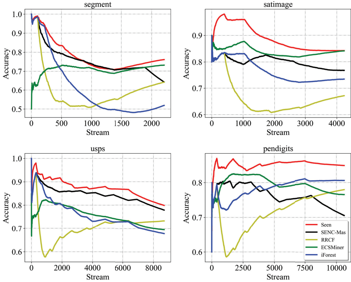
Figure 2: Accuracy results on the data streams of four datasets.
