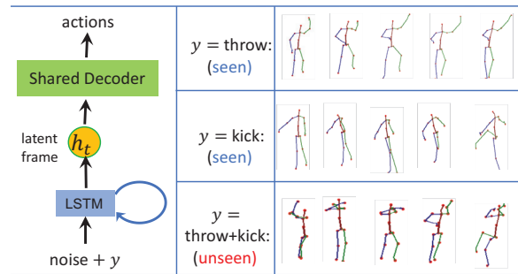
Figure 1: Generating sequences from pure noise, our model can learn smooth latent-frame transitions via an implicit LSTM-based RNN, which are then decoded to an action sequence via a shared decoder. The action sequence endsows a flexible implicit distribution induced by the input noise. Our model can not only generate actions whose class are seen during training (e.g., throw, kick), but also can generate actions of unseen mixed classes (e.g., throw+kick).
