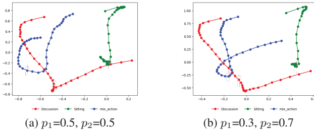
Figure 7: Latent space of mixed classes of actions with different mixing proportions p_1 and p_2 .
