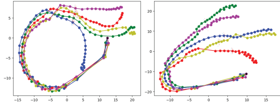
Figure 4: Action diversity of generated latent trajectories. Left: Greeting; Right: Posing.
