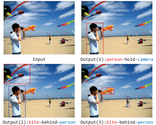
Figure 1: This figure shows some examples of visual relations from VRD dataset. Local information is insufficient for accurate relation detection. For example, in the this image, only the content in object bounding boxes is not enough to decide the relative position between kite and person. Therefore, we propose a novel contextual embedding to prompt global-local information interaction for relation detection.
